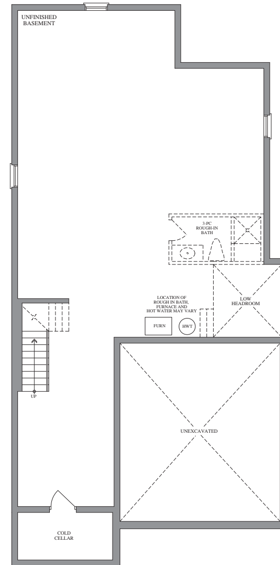
BASEMENT ELEVATION A & B
