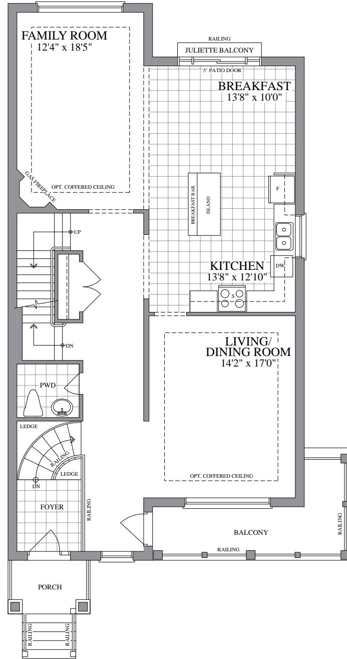
FIRST FLOOR ELEVATION A & B
