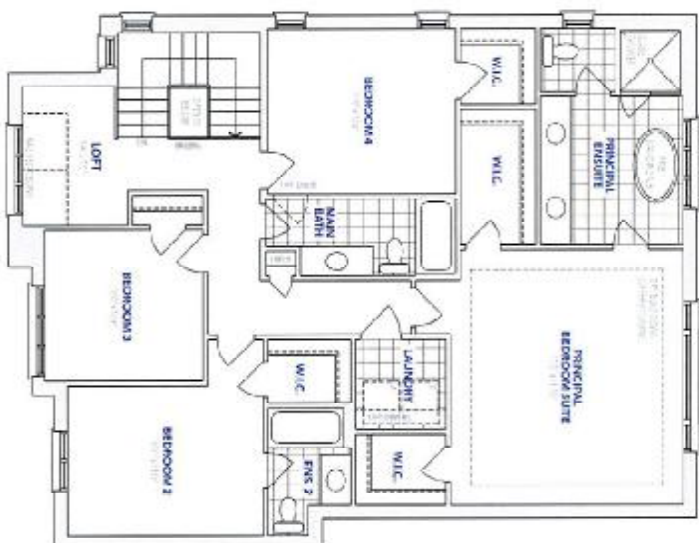
A SECOND FLOOR
