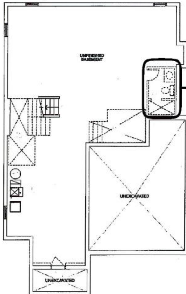
A BASEMENT
