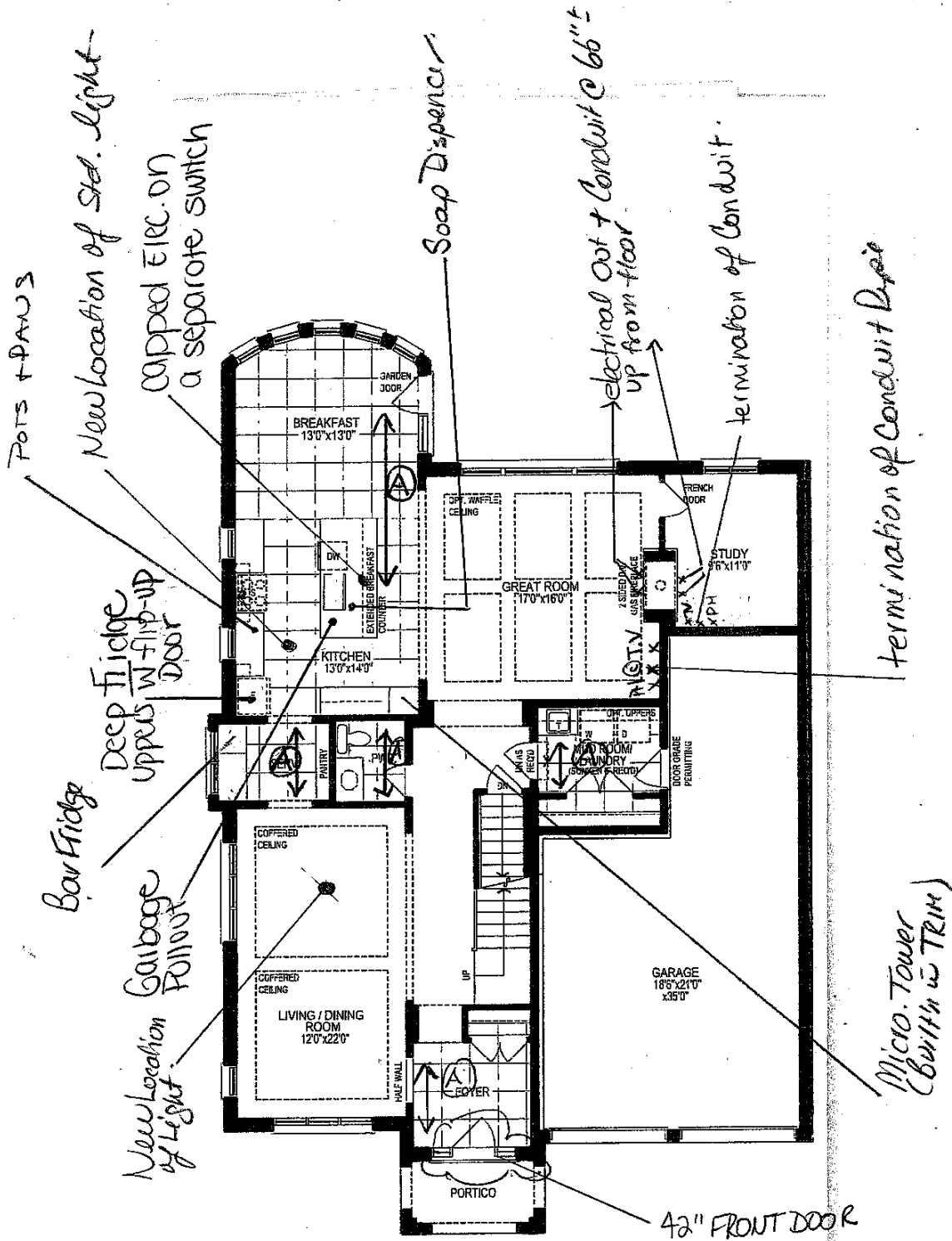
GROUND FLOOR PLAN 'B' - LOT 27
