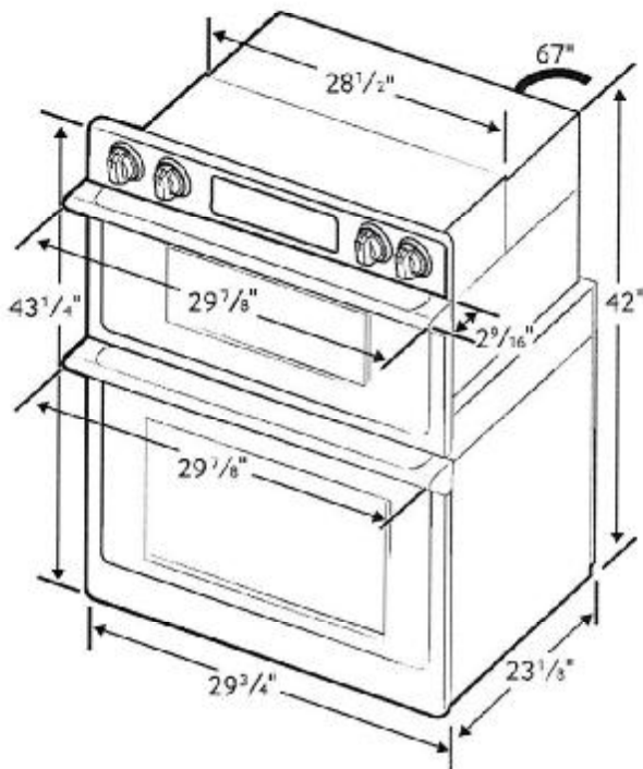
Product Dimensions
