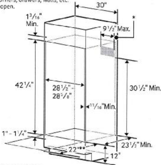
Product Dimensions
