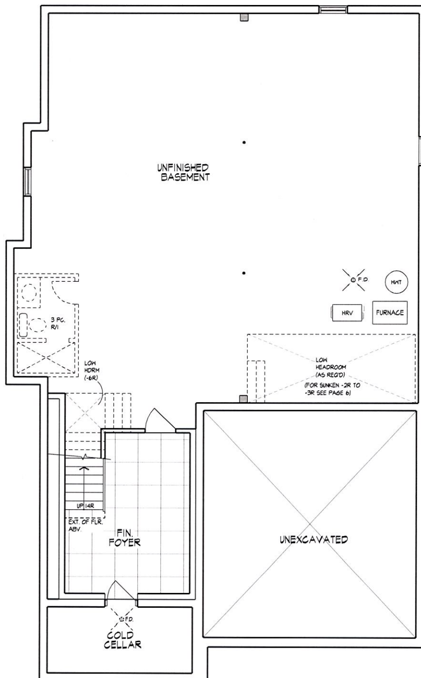
BASEMENT PLAN
