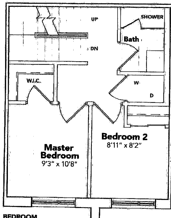
BEDROOM LEVEL
