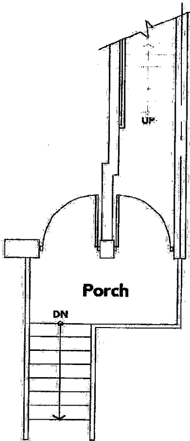
ENTRANCE LEVEL
