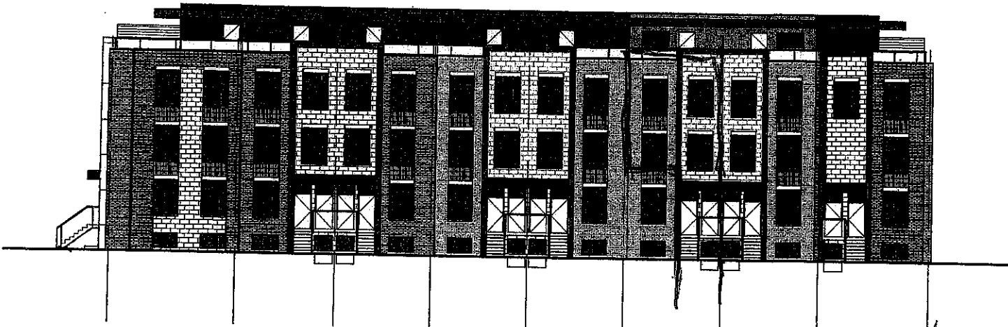
West Elevation - Block 1
