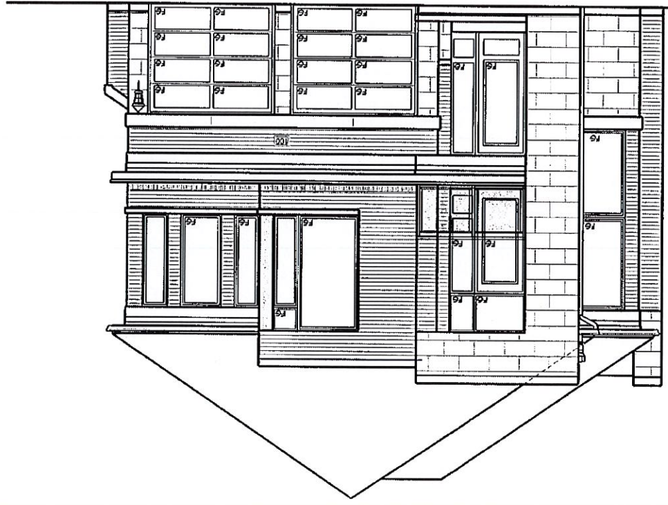
FRONT ELEVATION
