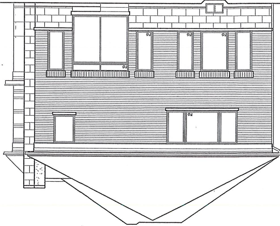
REAR ELEVATION
