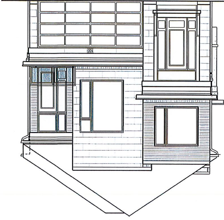
FRONT ELEVATION 'C'
