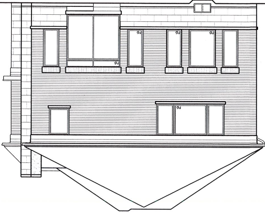
REAR ELEVATION
