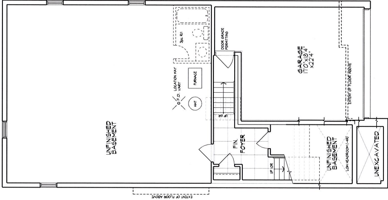
BASEMENT PLAN
