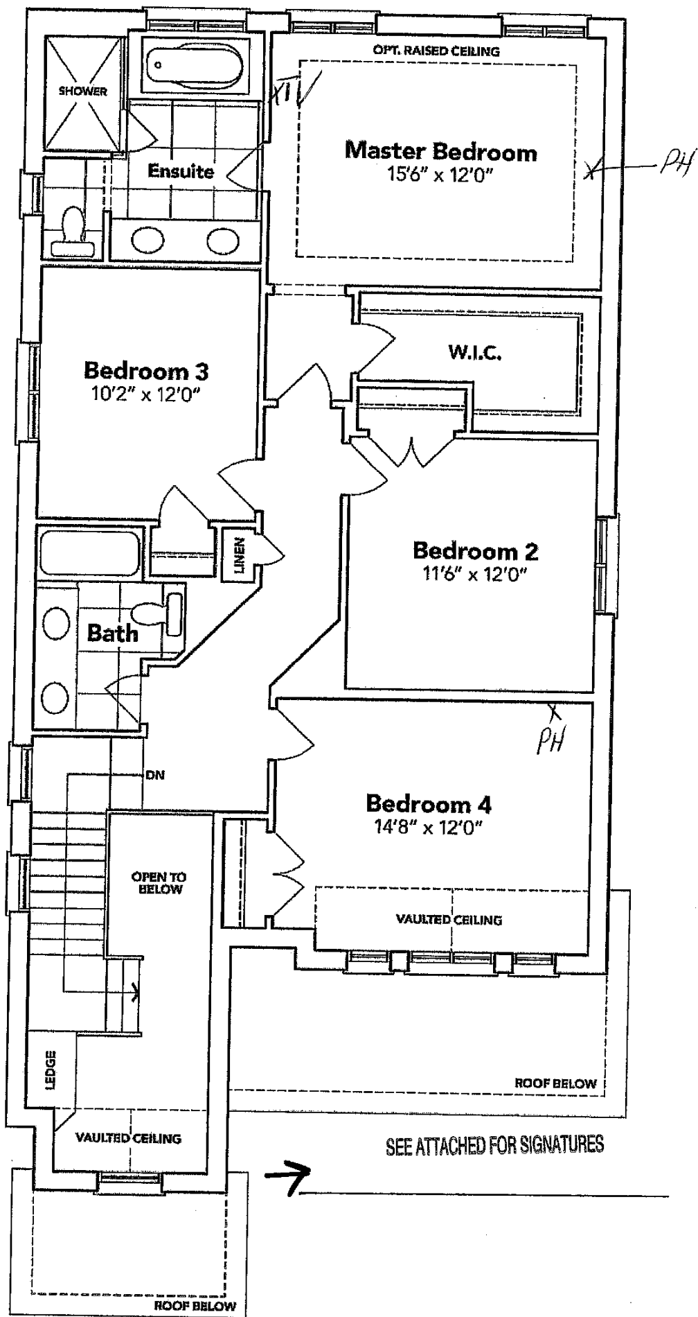
SECOND FLOOR EL. A
