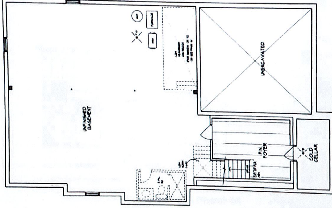
BASEMENT PLAN
