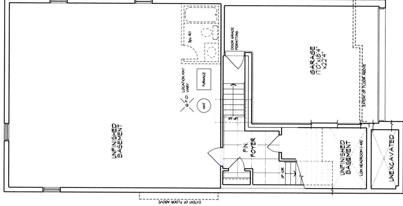
BASEMENT PLAN
