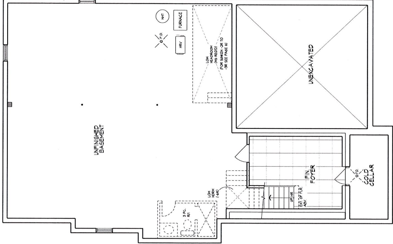
BASEMENT PLAN
