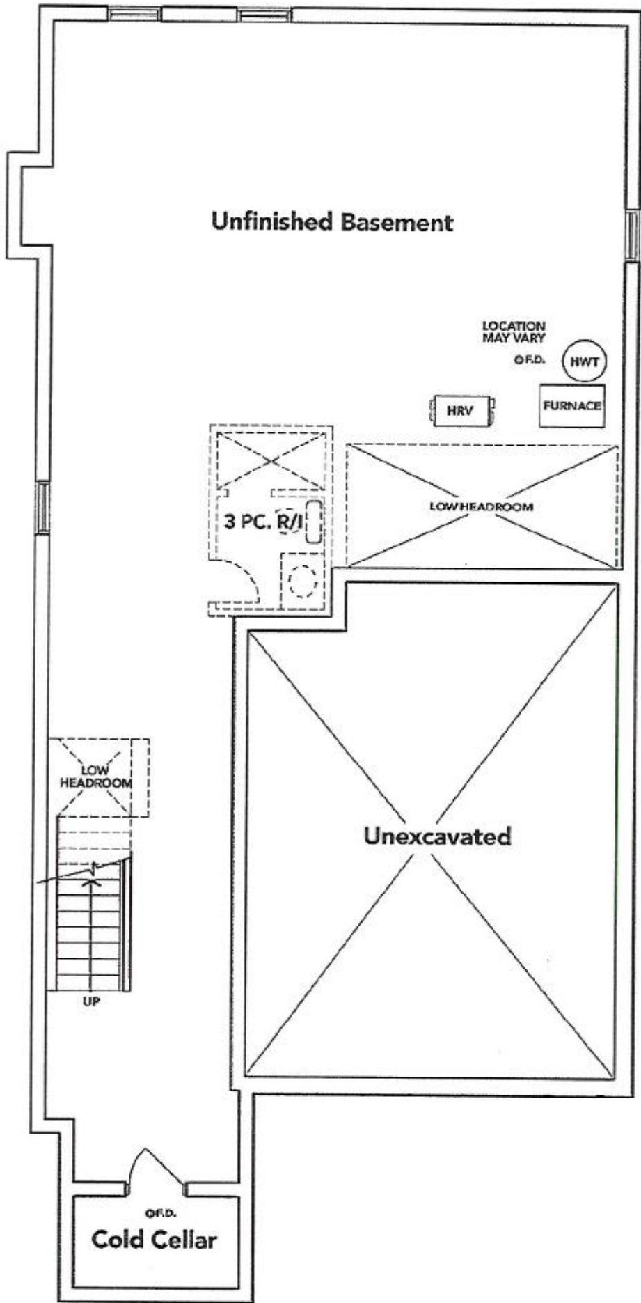
BASEMENT EL. A
