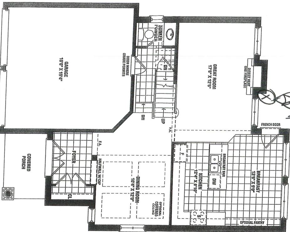
GROUND FLOOR ELEV. 'B'
