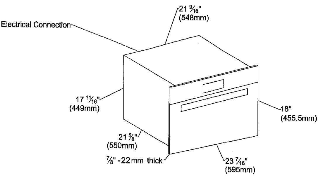
Isometric View
