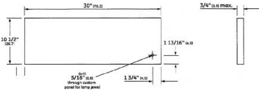
CUSTOM PANEL PREPARATION FRONT VIEW
