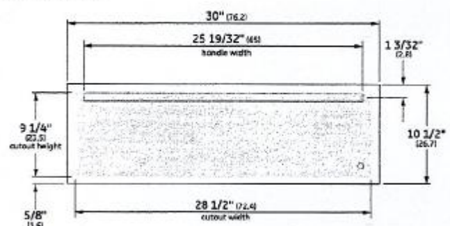
FRONT VIEW (SHOWING CUTOUT OVERLAP)
