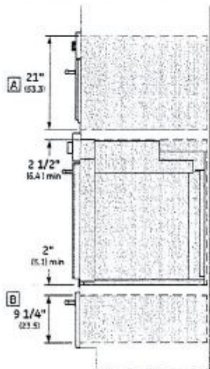
STANDARD INSTALLATION SIDE VIEW
