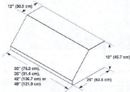
WITH FULL WIDTH DUCT COVER
