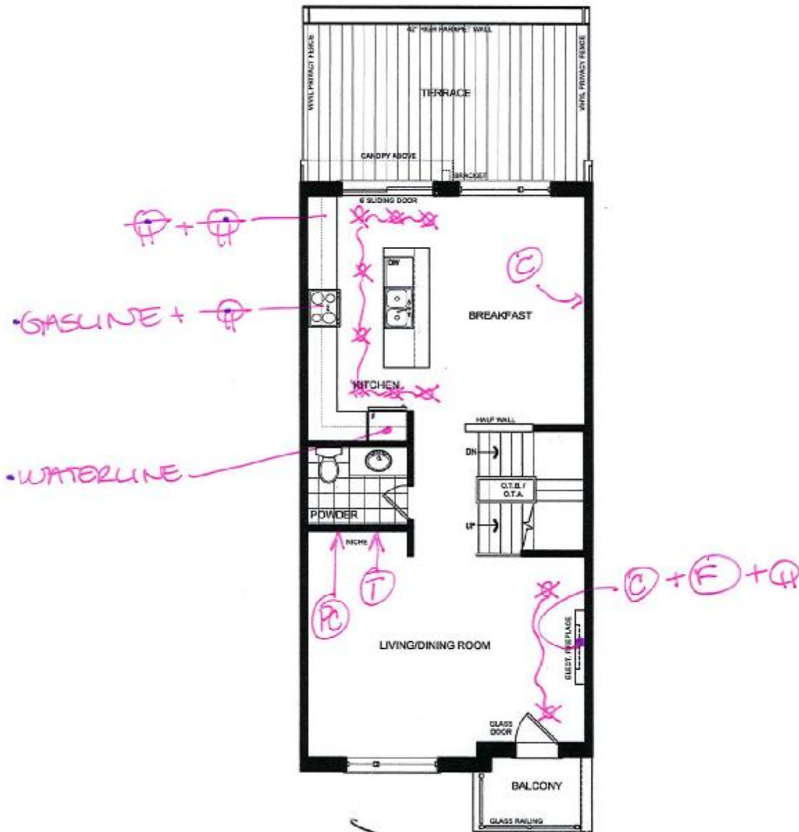
MAIN FLOOR ELEV 'B'
