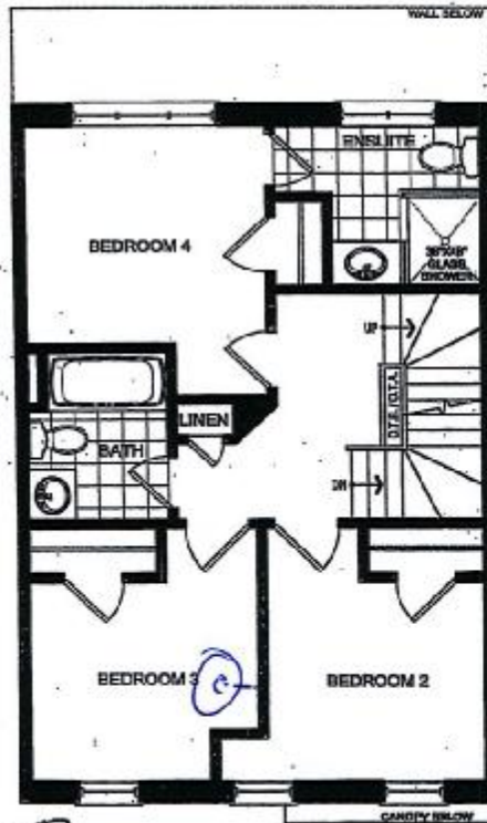
SECOND FLOOR ELEV. 'A'
