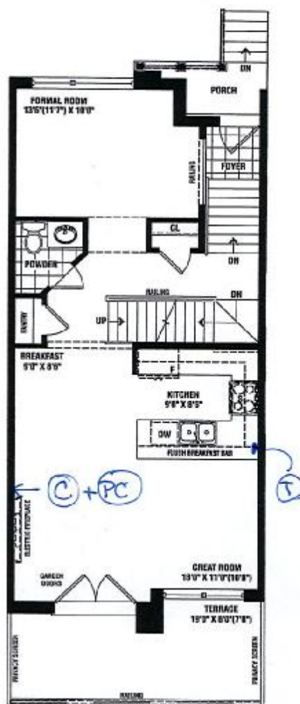
MAIN FLOOR
