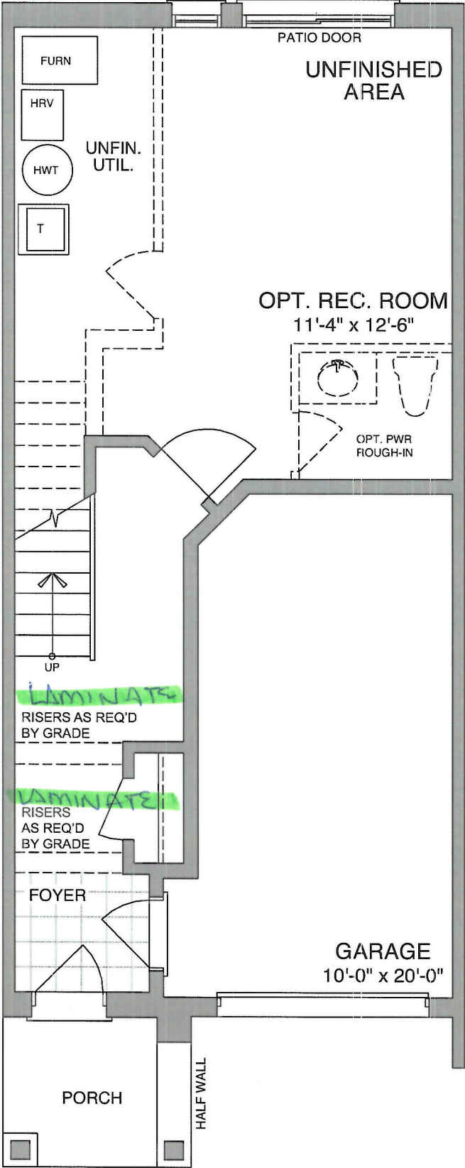
GROUND FLOOR - ELEV B
