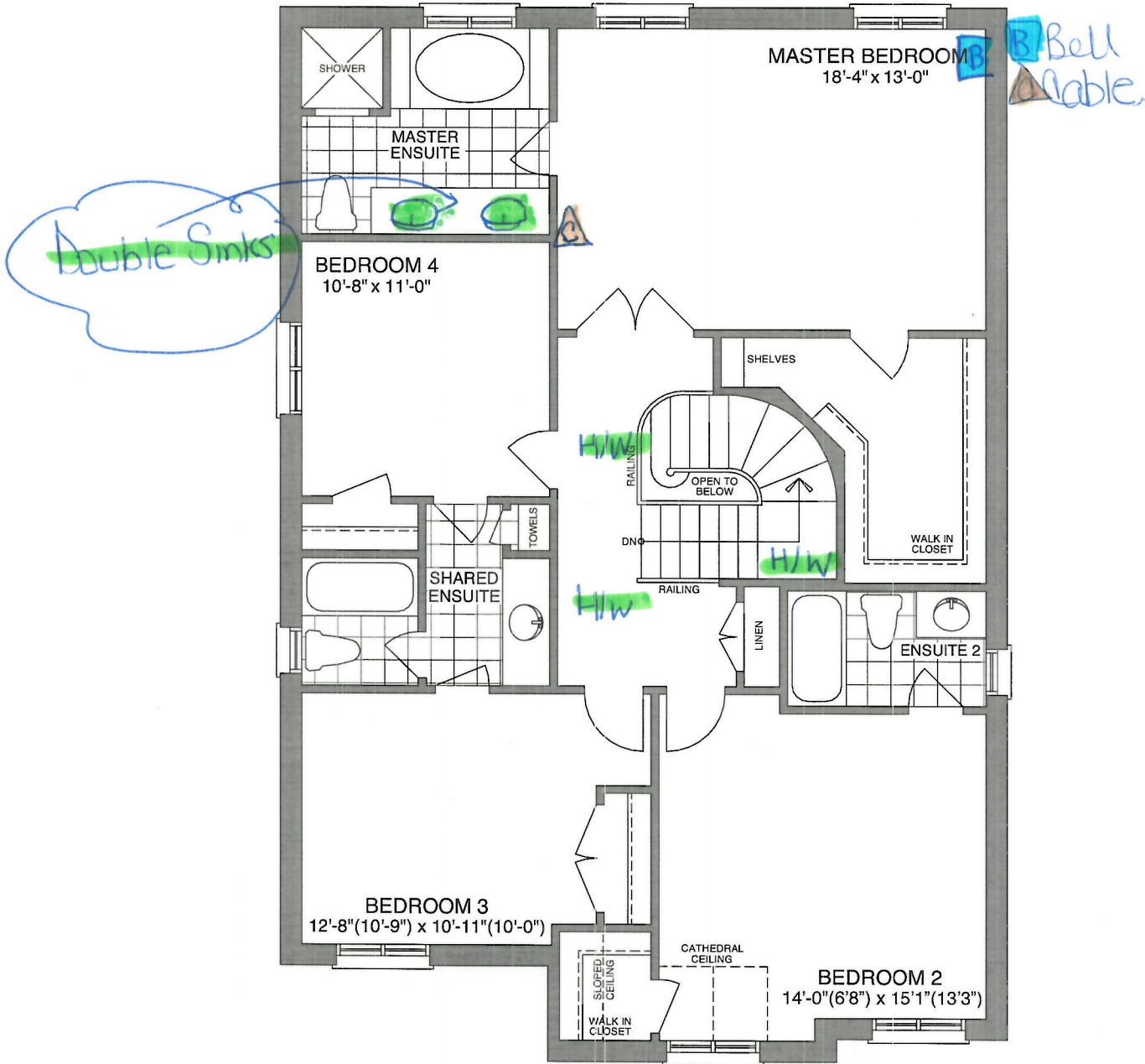
OPT. SECOND FLOOR - ELEV A
