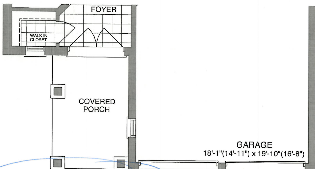
MAIN FLOOR - ELEV B
