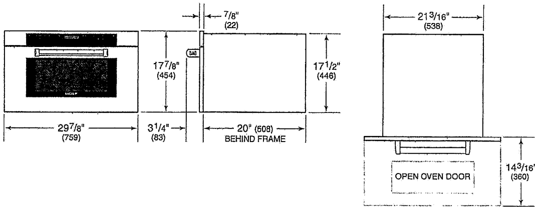
OVERALL DIMENSIONS
