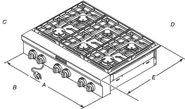
A. 36" (91.4 cm) cooktop: 29 1/8" (75.9 cm) 36" (91.4 cm) cooktop: 35 1/8" (91.1 cm) 48" (121.9 cm) cooktop: 47 1/8" (121.6 cm) B. 36" (91.4 cm) long 3 prong grounding-type power supply cord C. Model/serial rating plate (located on the underside of the cooktop burner base) D. Island trim or optional backguard E. 27 3/4" (70.5 cm)
