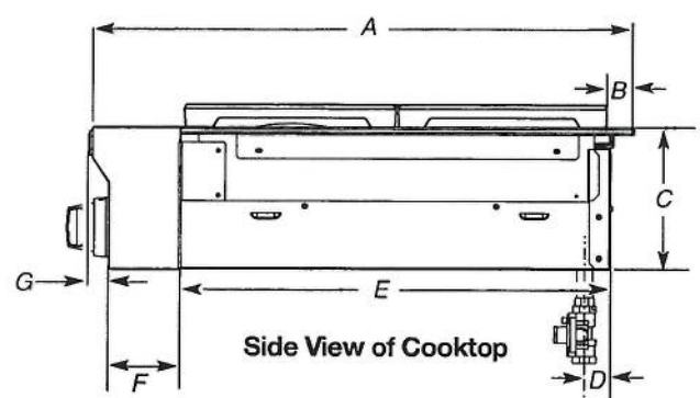
A. 27 3/4" (70.5 cm) B. 1 1/4" (3.2 cm) C. 7 1/16" (18.8 cm) D. Gas inlet is located 1 7/8" (4.8 cm) from the back of the cooktop burner base and 4 7/8" (12.4 cm) in from left-hand side of the cooktop burner base. E. 22" (55.9 cm) F. 3 3/8" (9.2 cm) G. 1" (2.6 cm)
