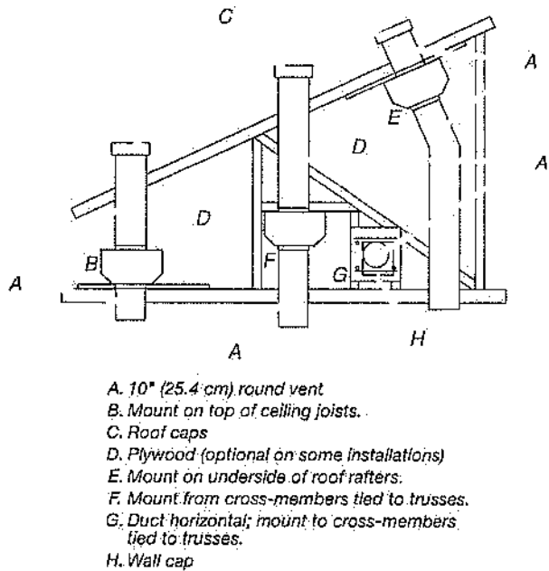
Typical In-line Blower Motor System Venting Installations
