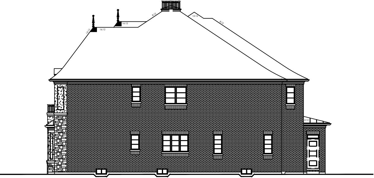
RIGHT SIDE ELEVATION 'C'
