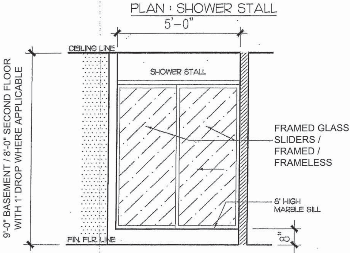
PART.ELEV. : SHOWER STALL
