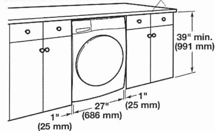
Recessed area or closet installation (washer only)
