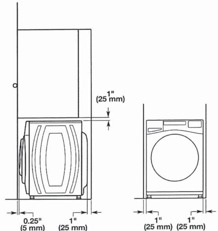
Custom cabinet installation
