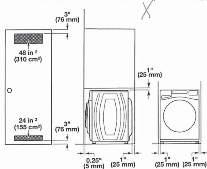
Recessed area or closet installation (washer only)
