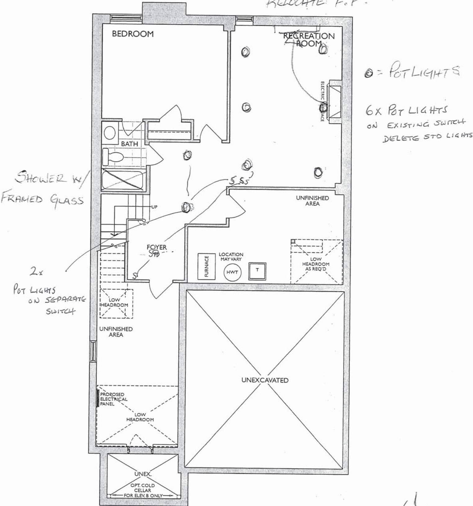
FINISHED LOWER LEVEL ELEV. A & B
