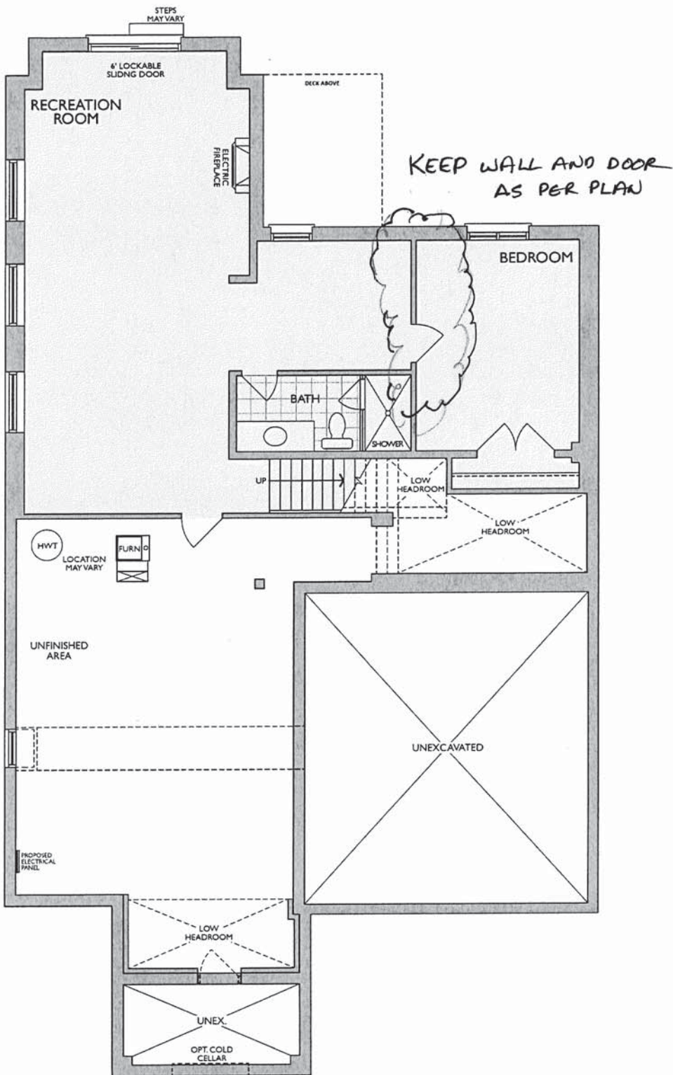
FINISHED LOWER LEVEL "WALK OUT" VERSION 1 ELEV. A & B
