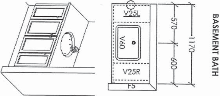
'SPACES' KITCHENETTE FINISHED LOWER LEVEL
