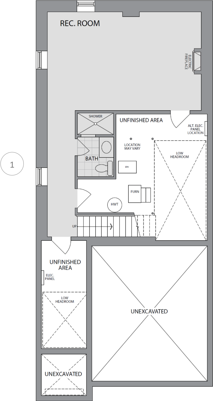
FINISHED LOWER LEVEL ELEVATION A, B & C
