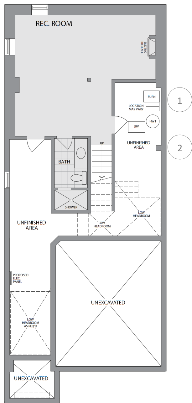
FINISHED LOWER LEVEL ELEVATION B
