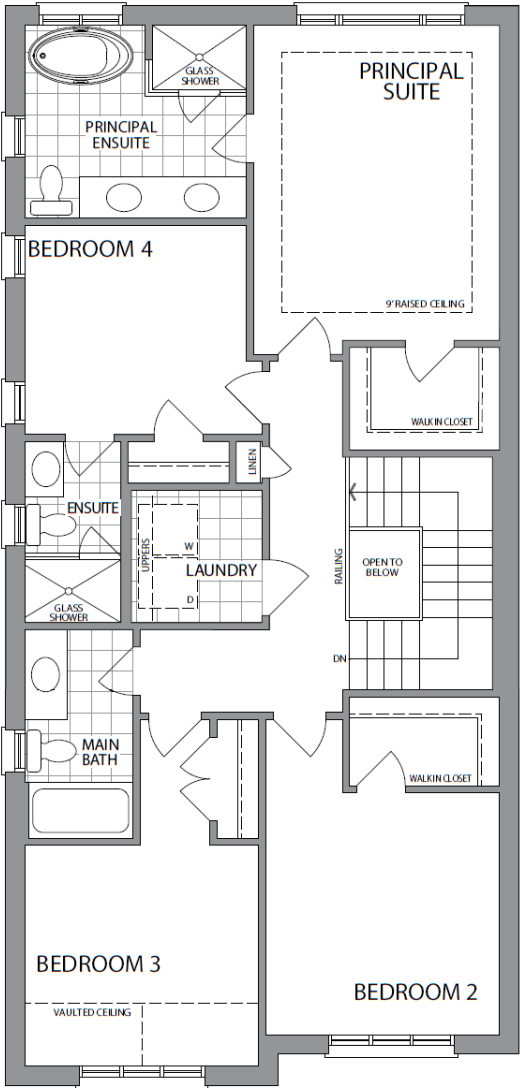
SECOND LEVEL ELEVATION B
