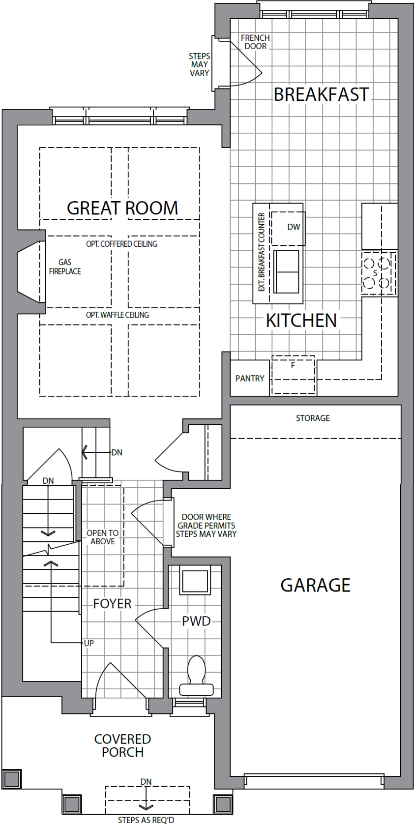
MAIN LEVEL ELEVATION C
