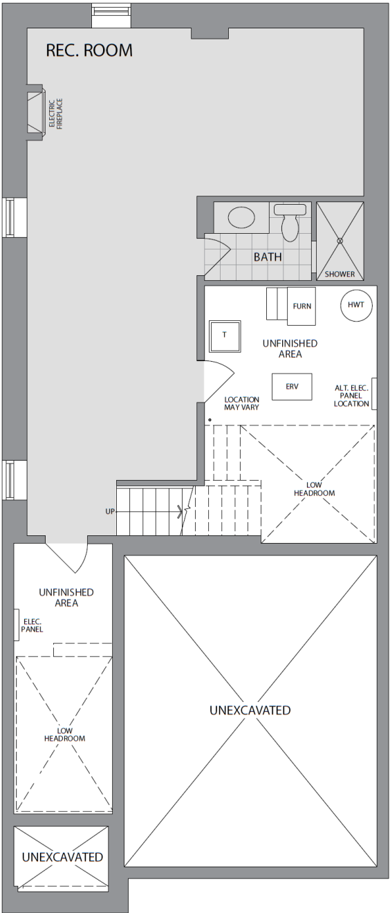
FINISHED LOWER LEVEL ELEVATION C
