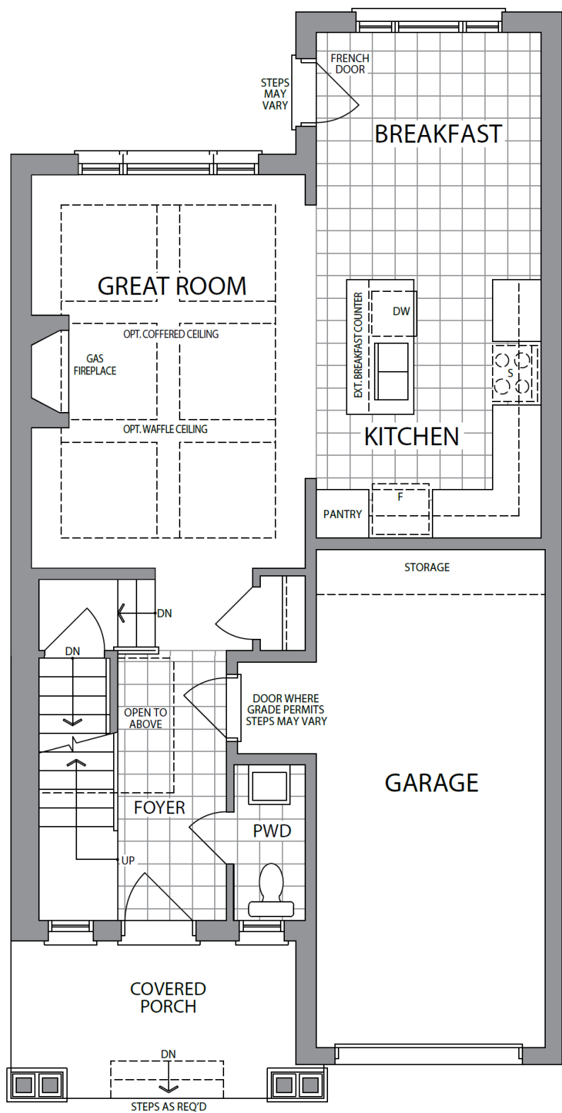
MAIN LEVEL ELEVATION B
