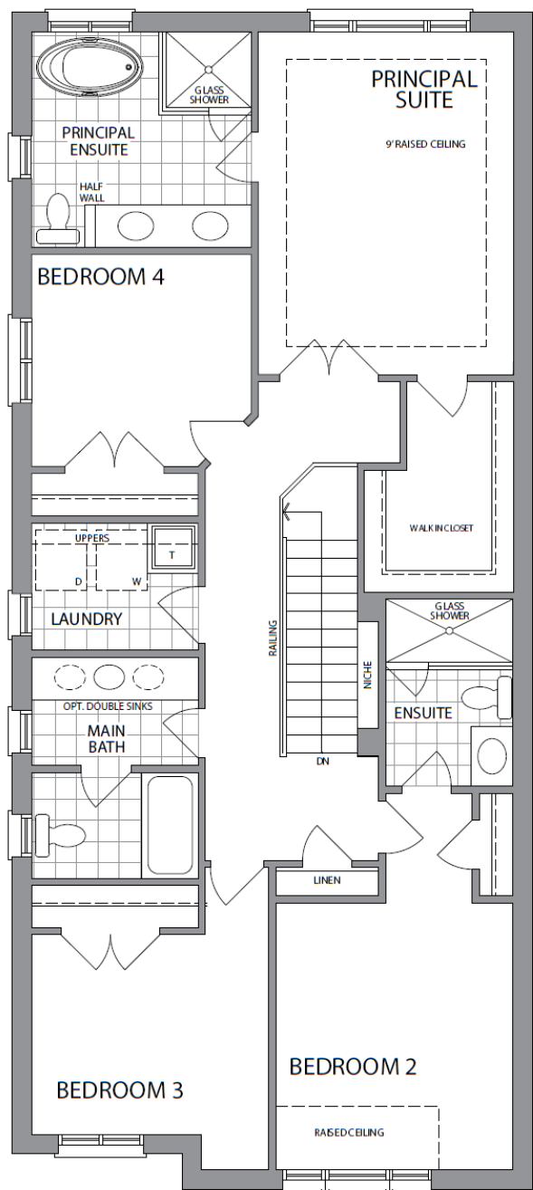
SECOND LEVEL ELEVATION A
