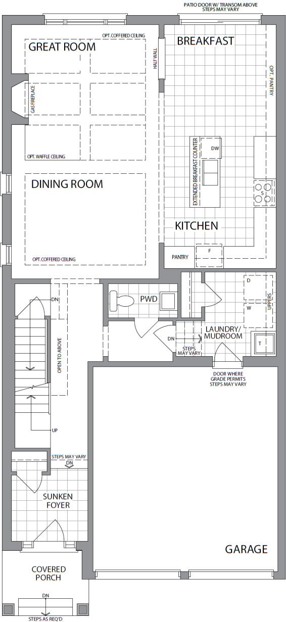
MAIN LEVEL ELEVATION B
