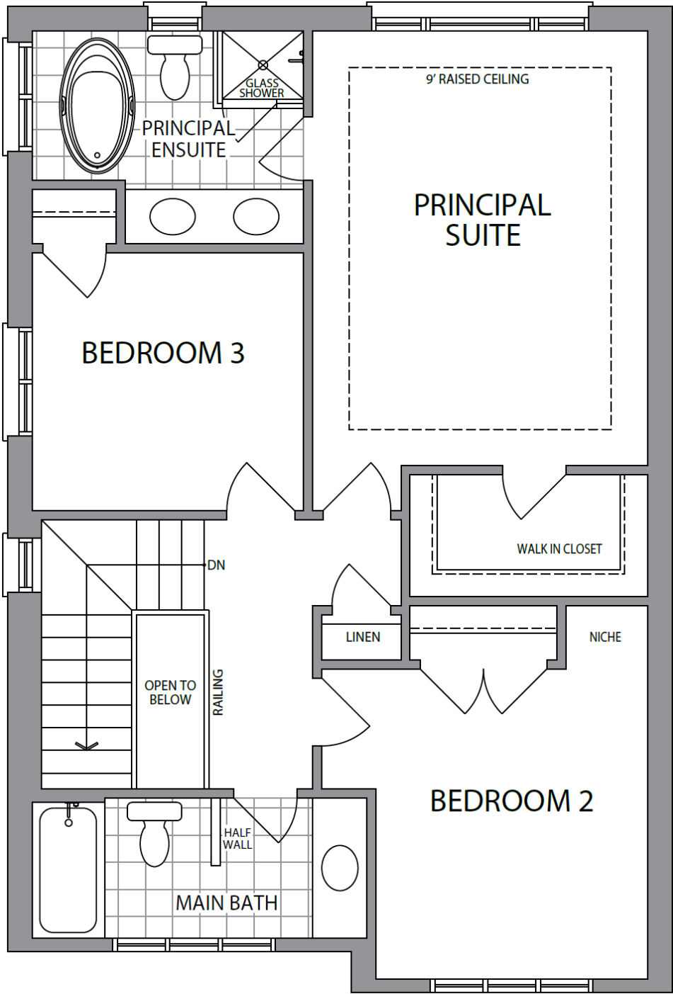
SECOND LEVEL ELEVATION A
