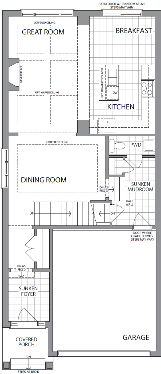
MAIN LEVEL ELEVATION A
