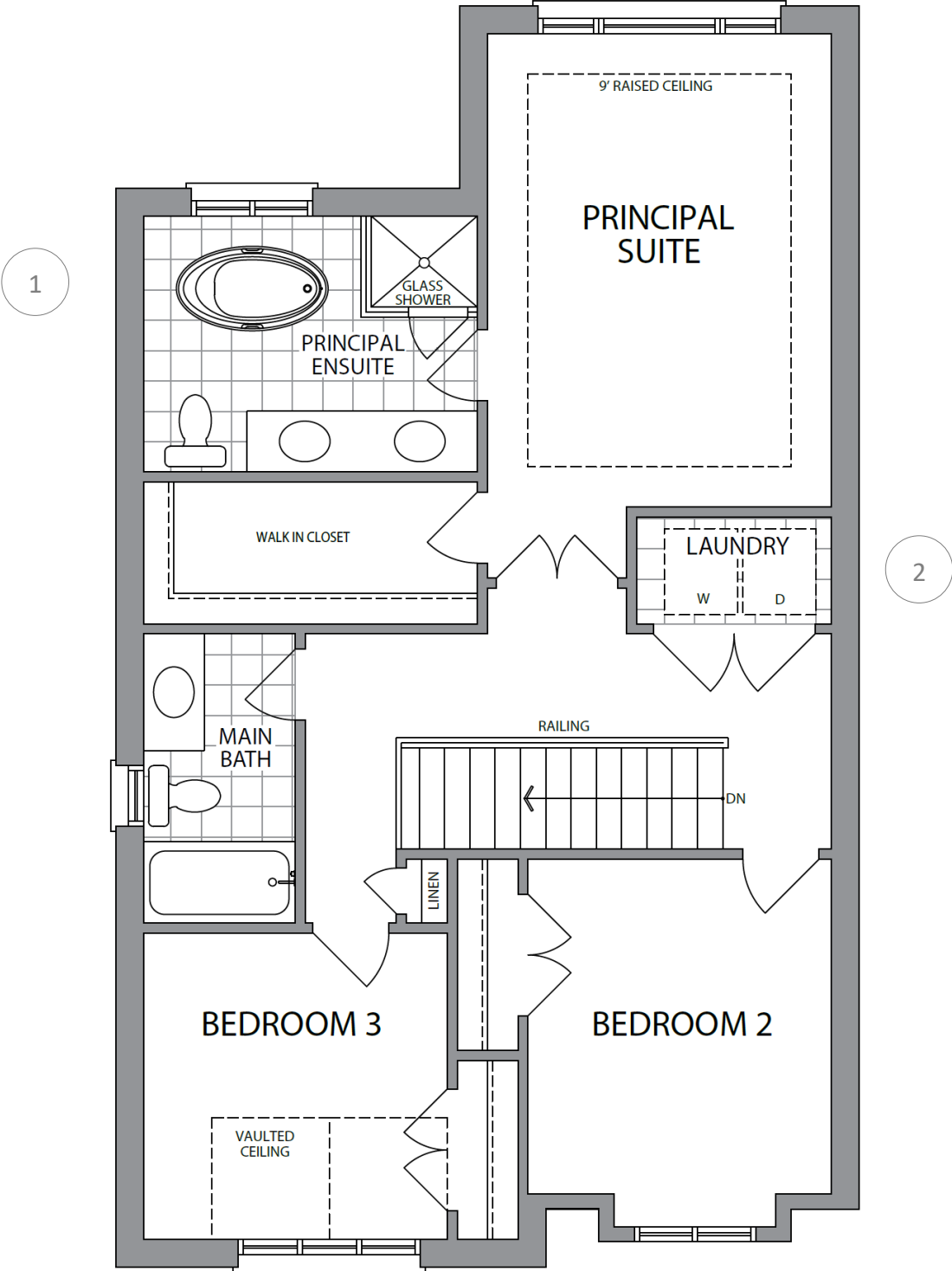
SECOND LEVEL ELEVATION A
