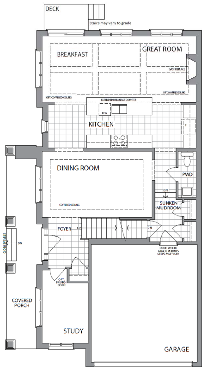
MAIN LEVEL ELEVATION C
