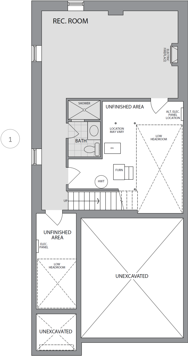
FINISHED LOWER LEVEL ELEVATION A, B & C
