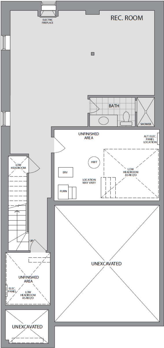
FINISHED LOWER LEVEL ELEVATION A
