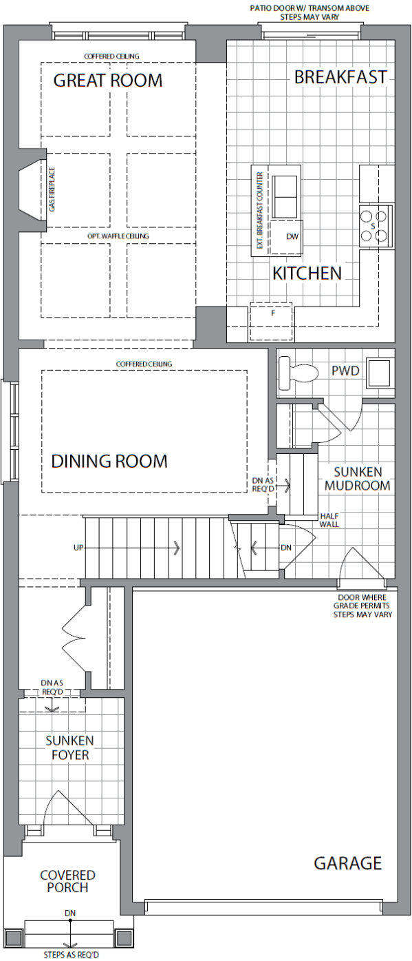
MAIN LEVEL ELEVATION C
