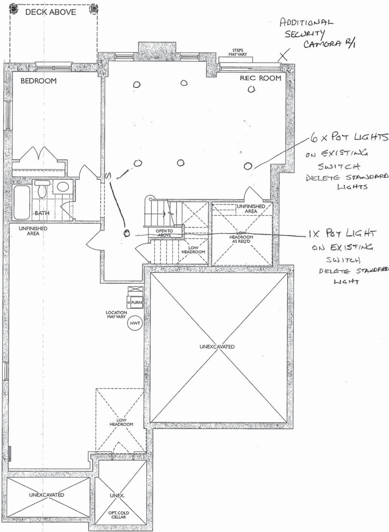
LOWER LEVEL - WALK OUT BASEMENT ELEV. A
