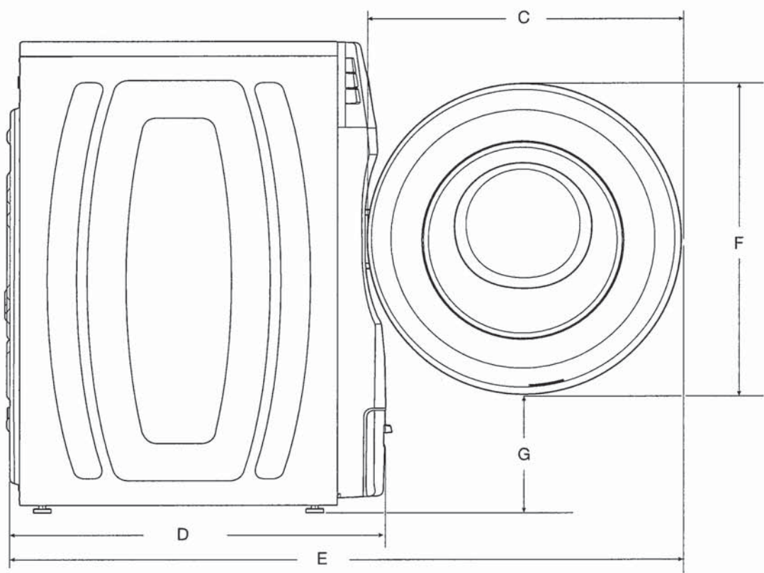
SIDE VIEW
