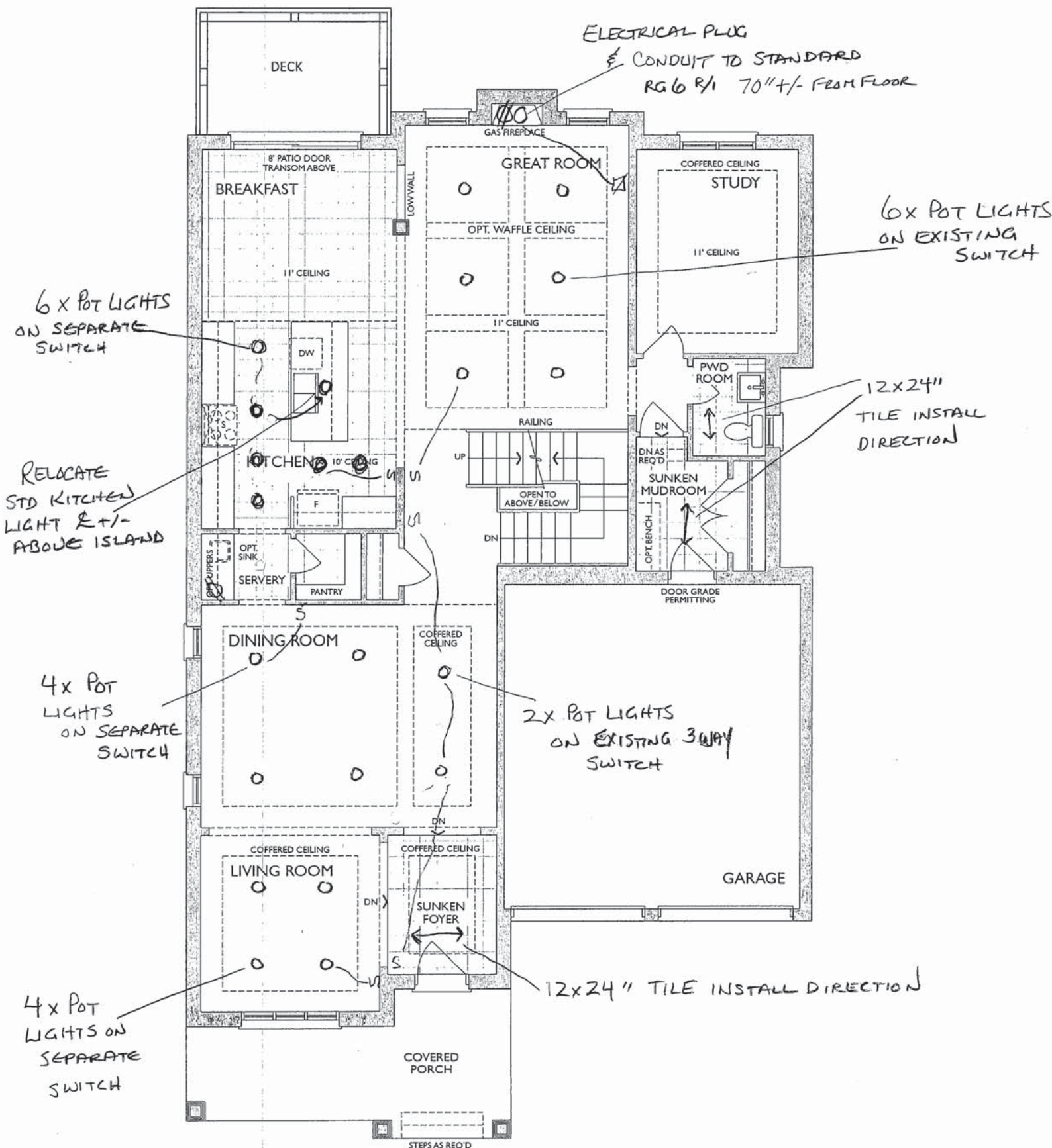
GROUND FLOOR - WALK OUT BASEMENT ELEV. A
