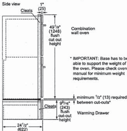
Flush installation Combination oven over storage or warming drawer Side view
