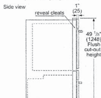
Standard Installation Combination oven over storage or warming drawer
