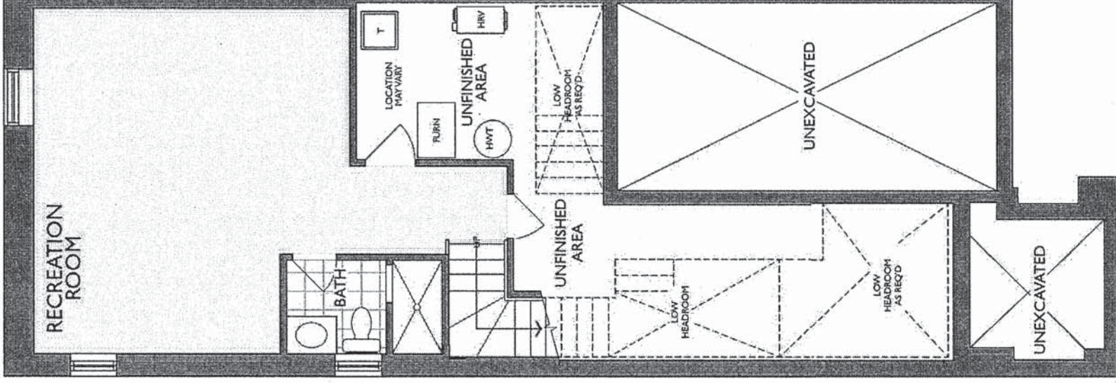
LOWER LEVEL ELEVATION B ~ END
