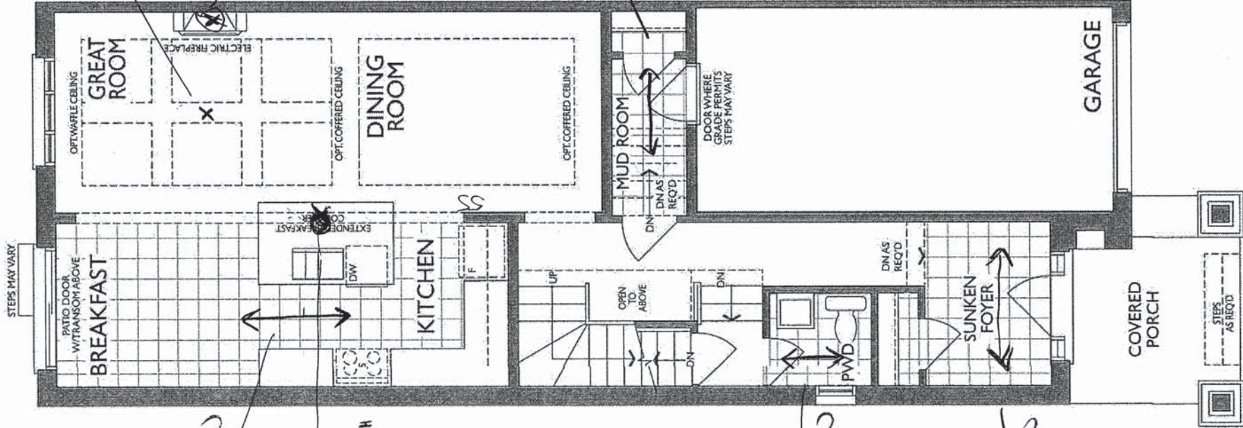
MAIN FLOOR ELEVATION B - END
