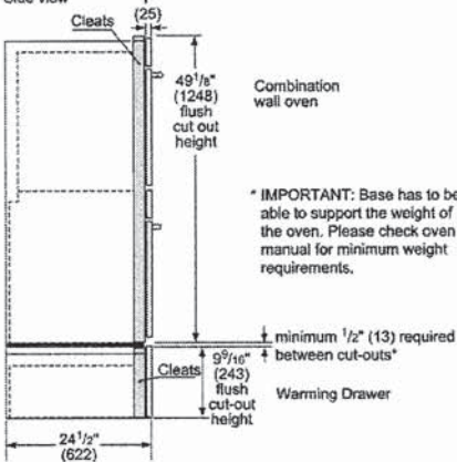
Flush installation Combination oven over storage or warming drawer Side view
