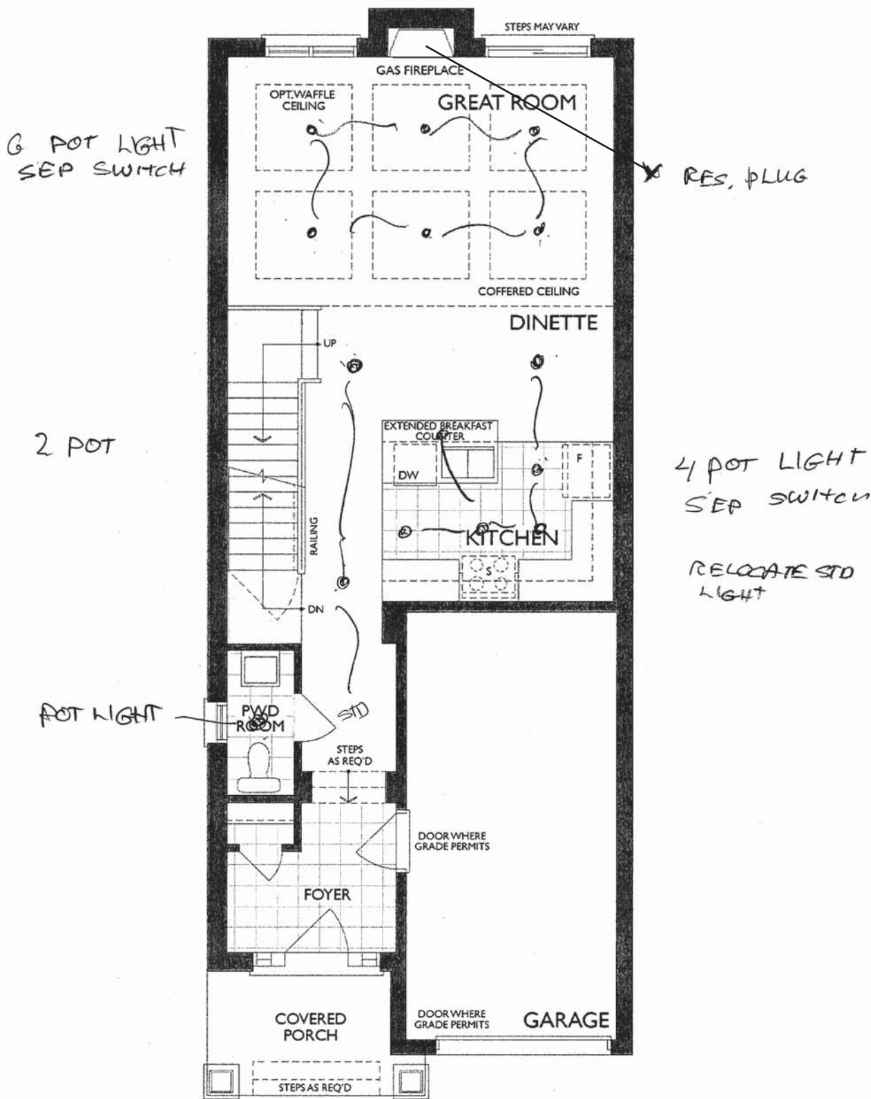
GROUND FLOOR ELEVATION 'A'
