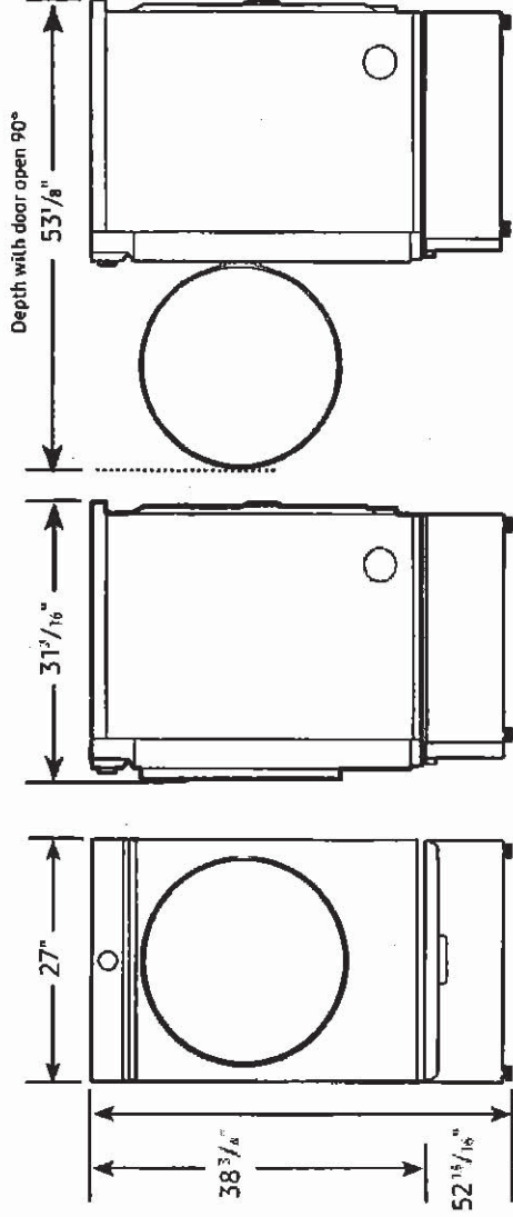
Dimensions Required dimensions for installation with pedestal:
