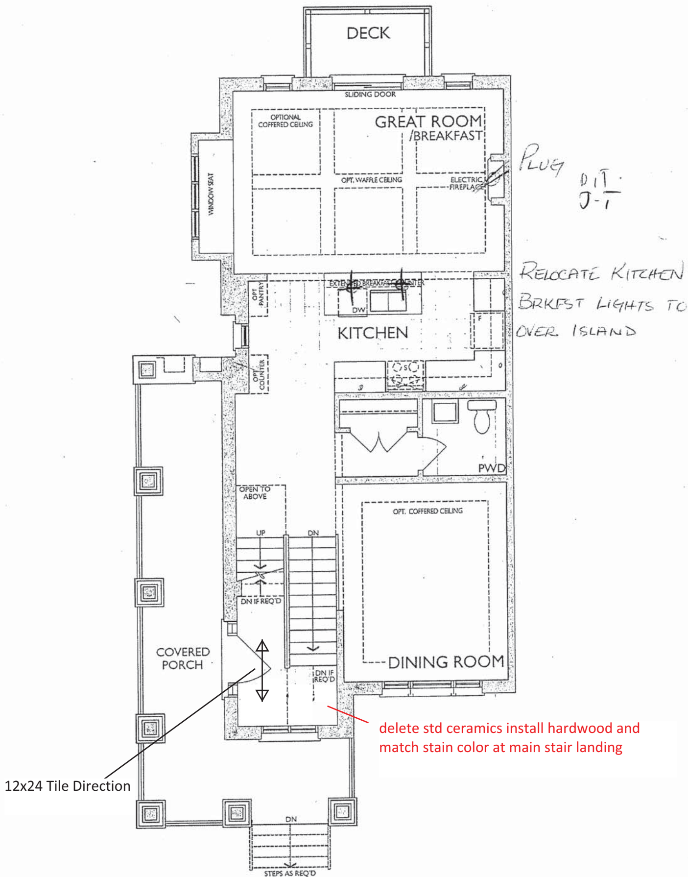
MAIN LEVEL ELEVATION A
