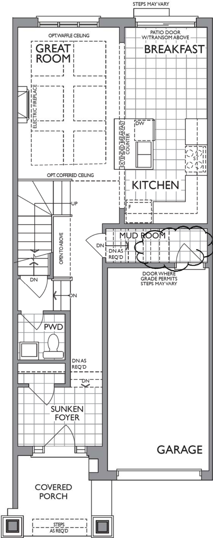
MAIN FLOOR ELEVATION A *Sunken condition
