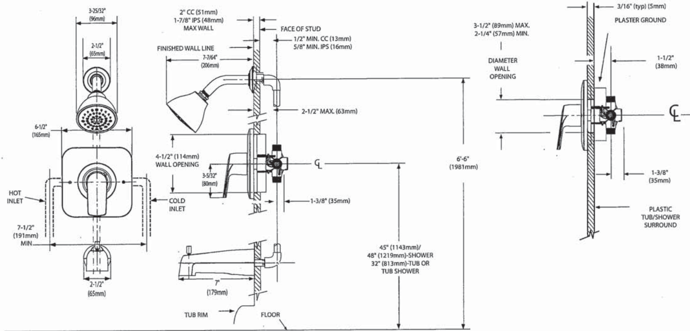
THICK WALL APPLICATION
