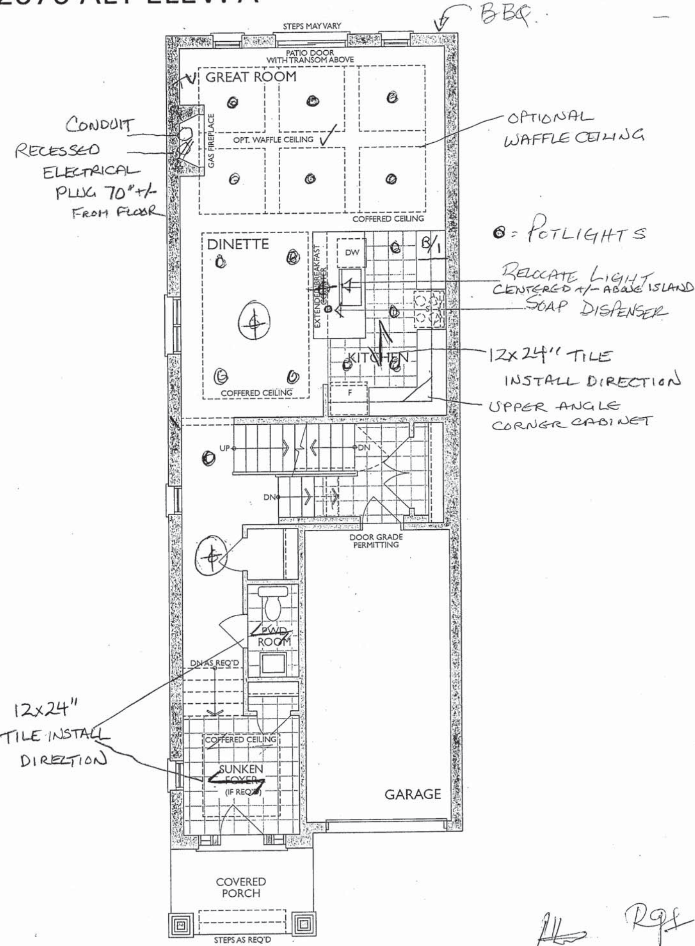
GROUND FLOOR ELEVATION A
