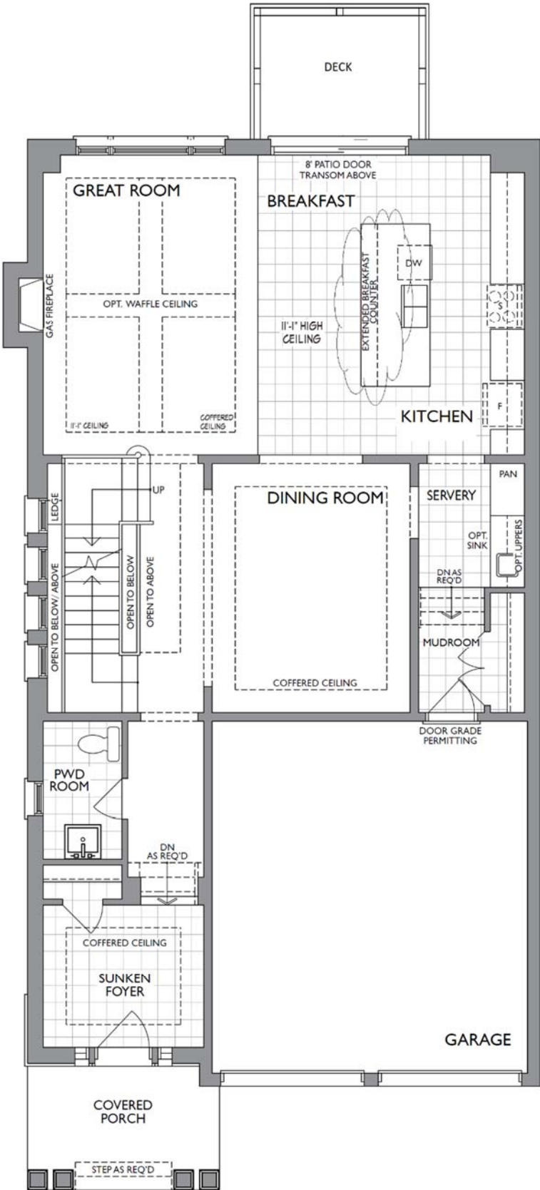
GROUND FLOOR - WALK OUT BASEMENT ELEV. A *Island Size Changed
