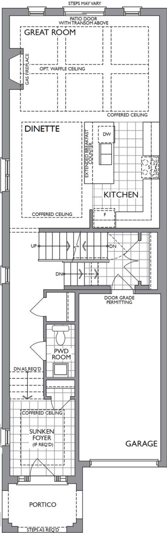
GROUND FLOOR ELEV. B
