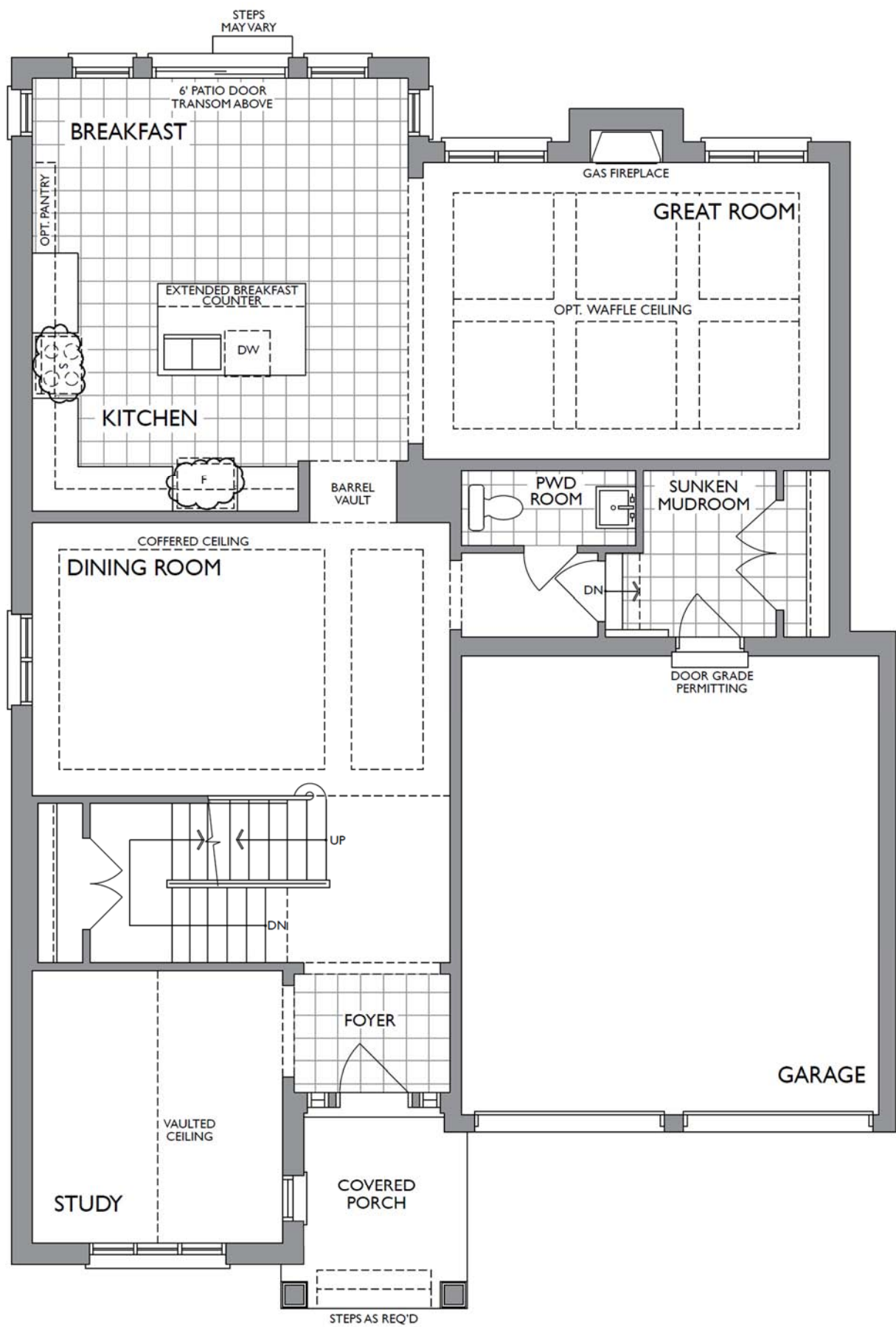
GROUND FLOOR ELEV. A
