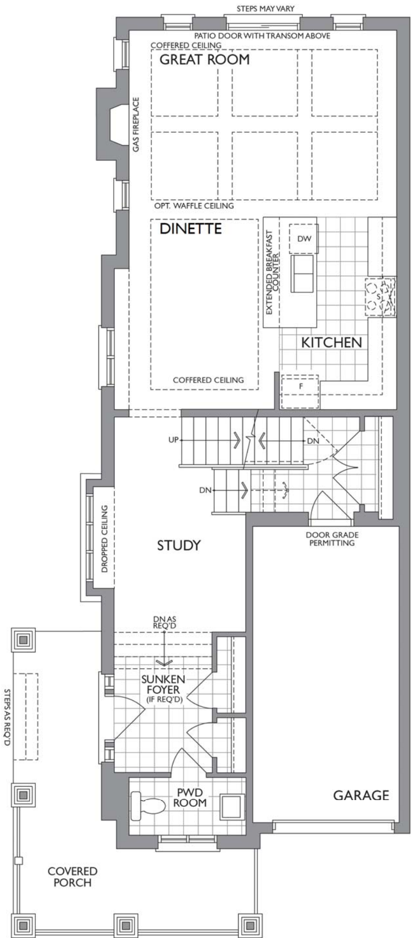
GROUND FLOOR ELEV. A CORNER
