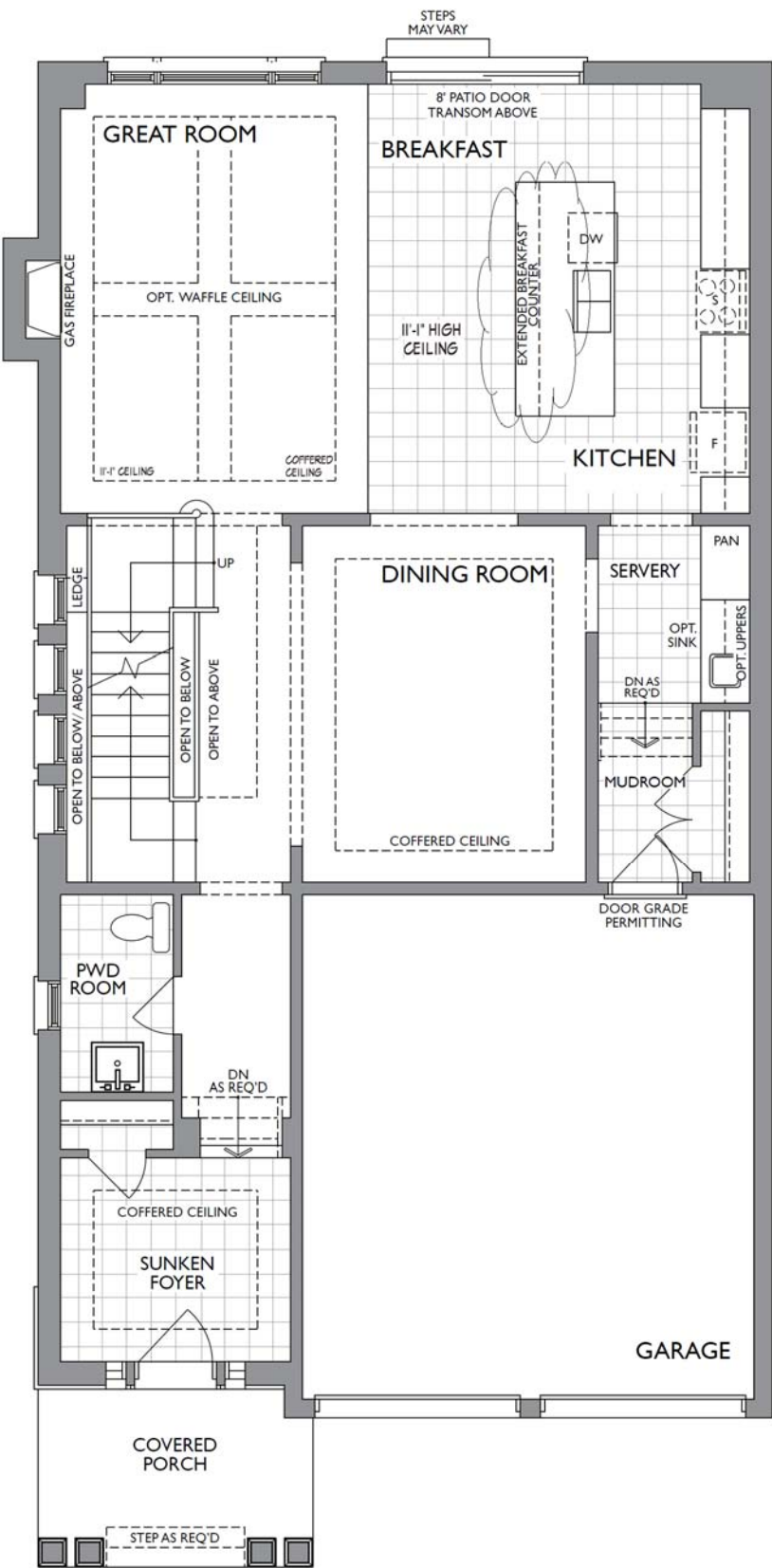
GROUND FLOOR ELEV. A *Island Size Changed
