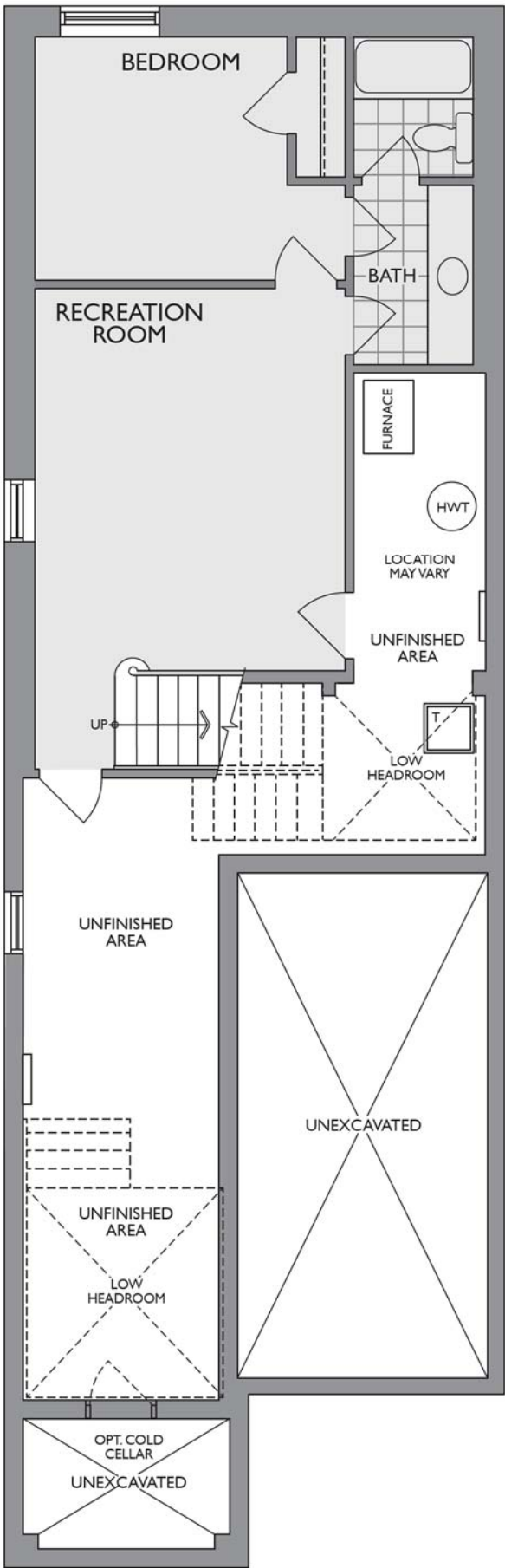
LOWER LEVEL ELEV. A
