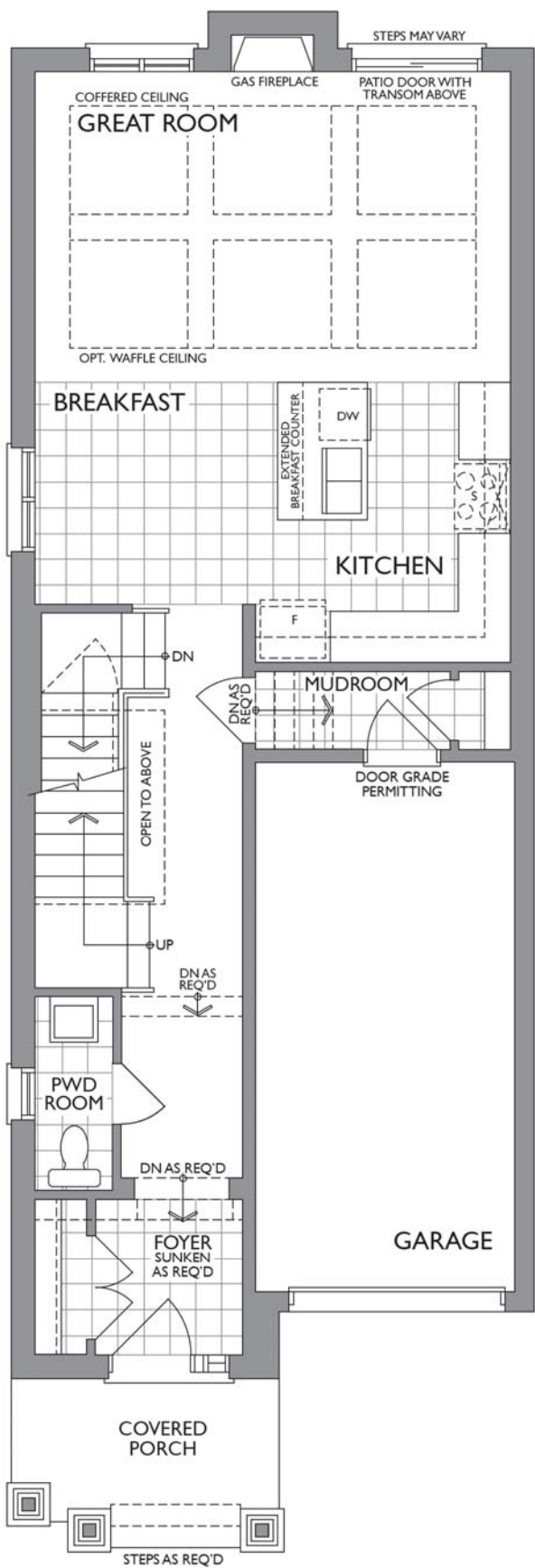
GROUND FLOOR ELEV. A
