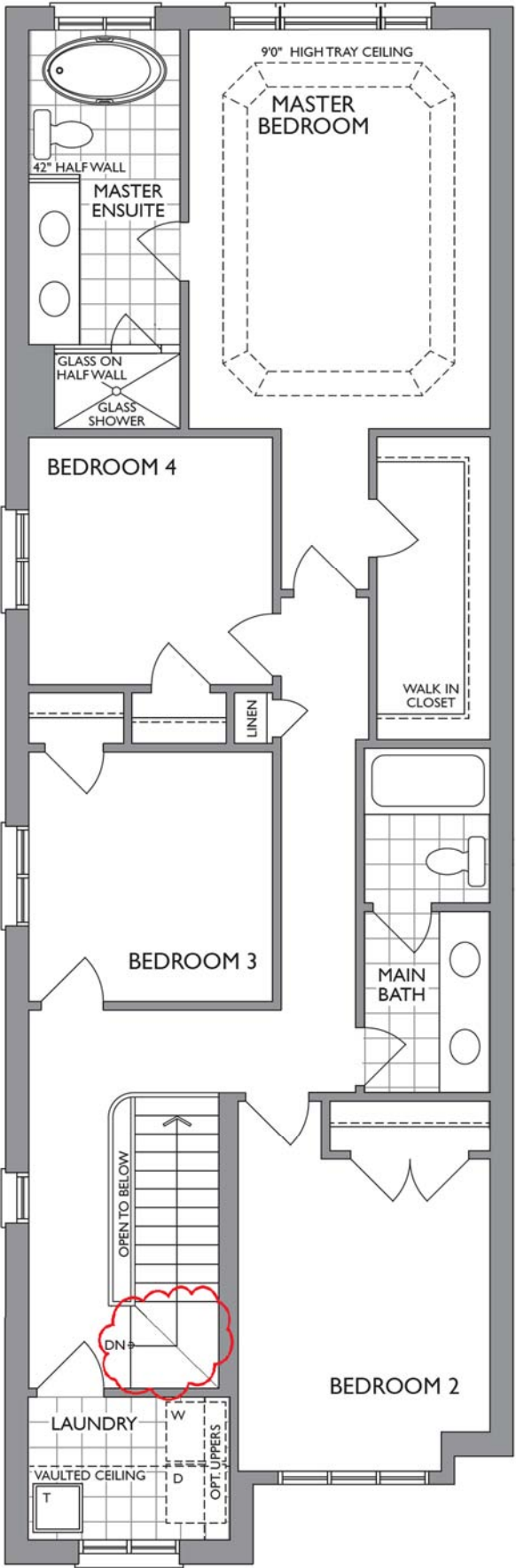
SECOND FLOOR ELEV. B
