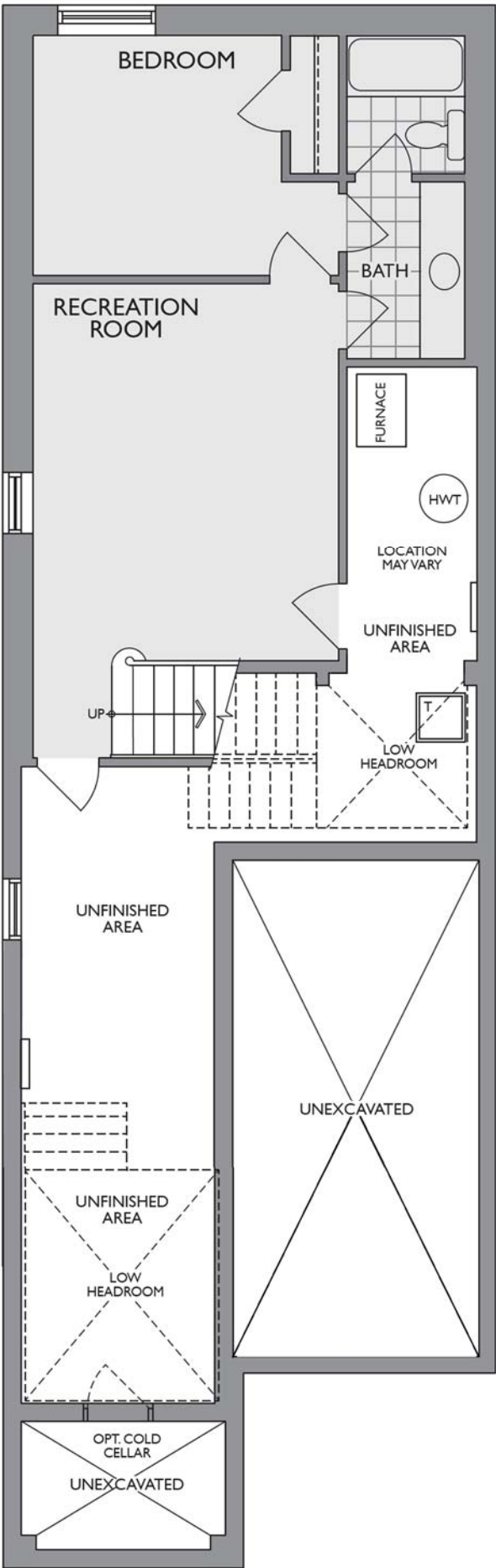
LOWER LEVEL ELEV. B
