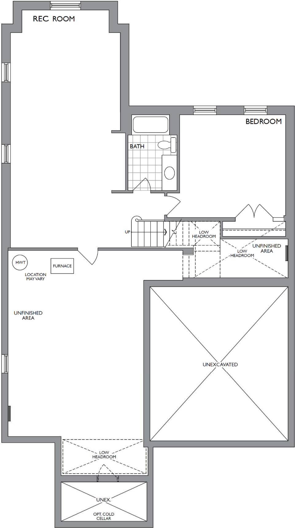
LOWER LEVEL ELEV. A & B
