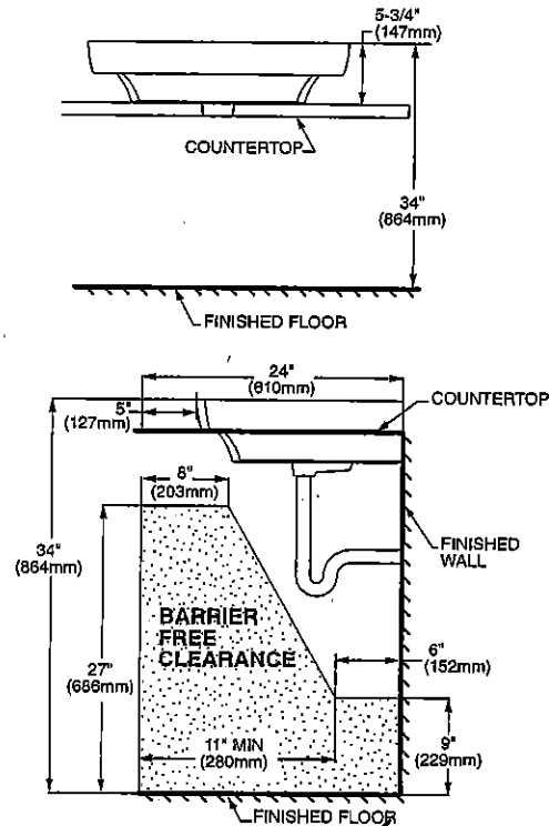
DROP-IN SINK CONFIGURATION
