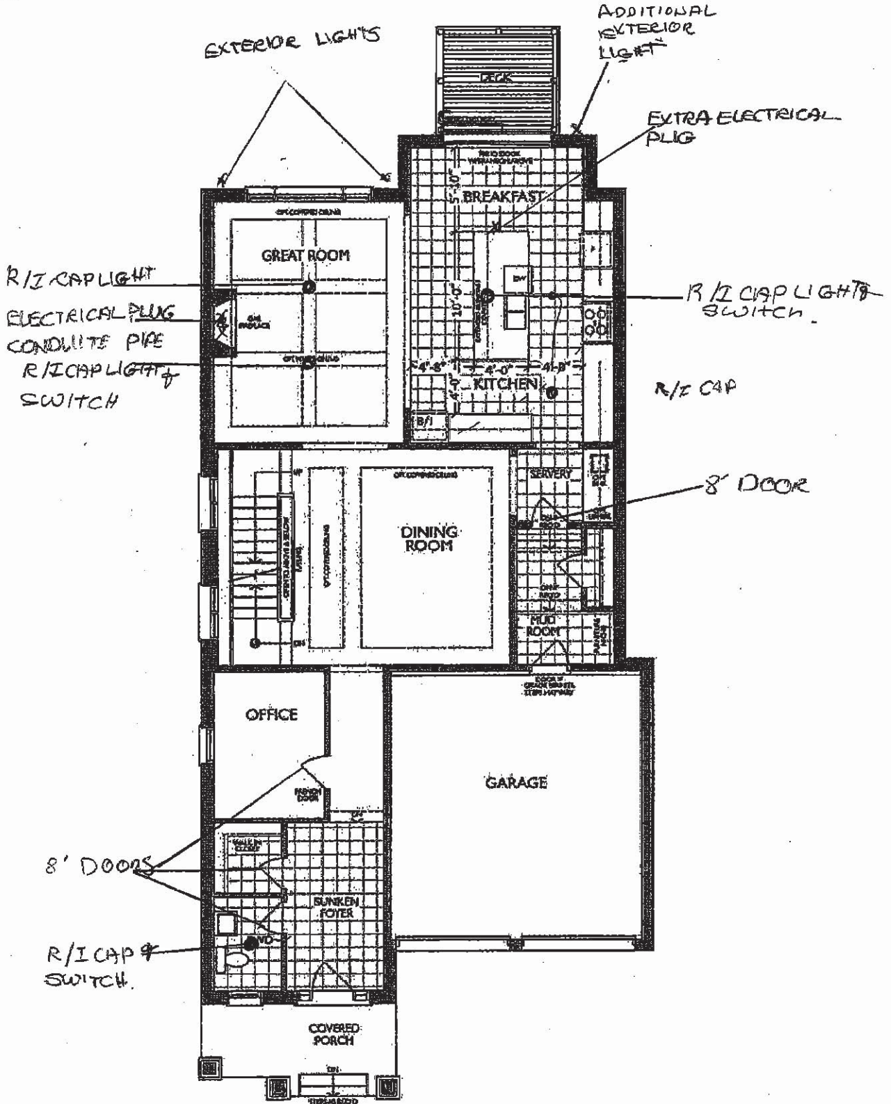
MAIN FLOOR ELEVATION A
