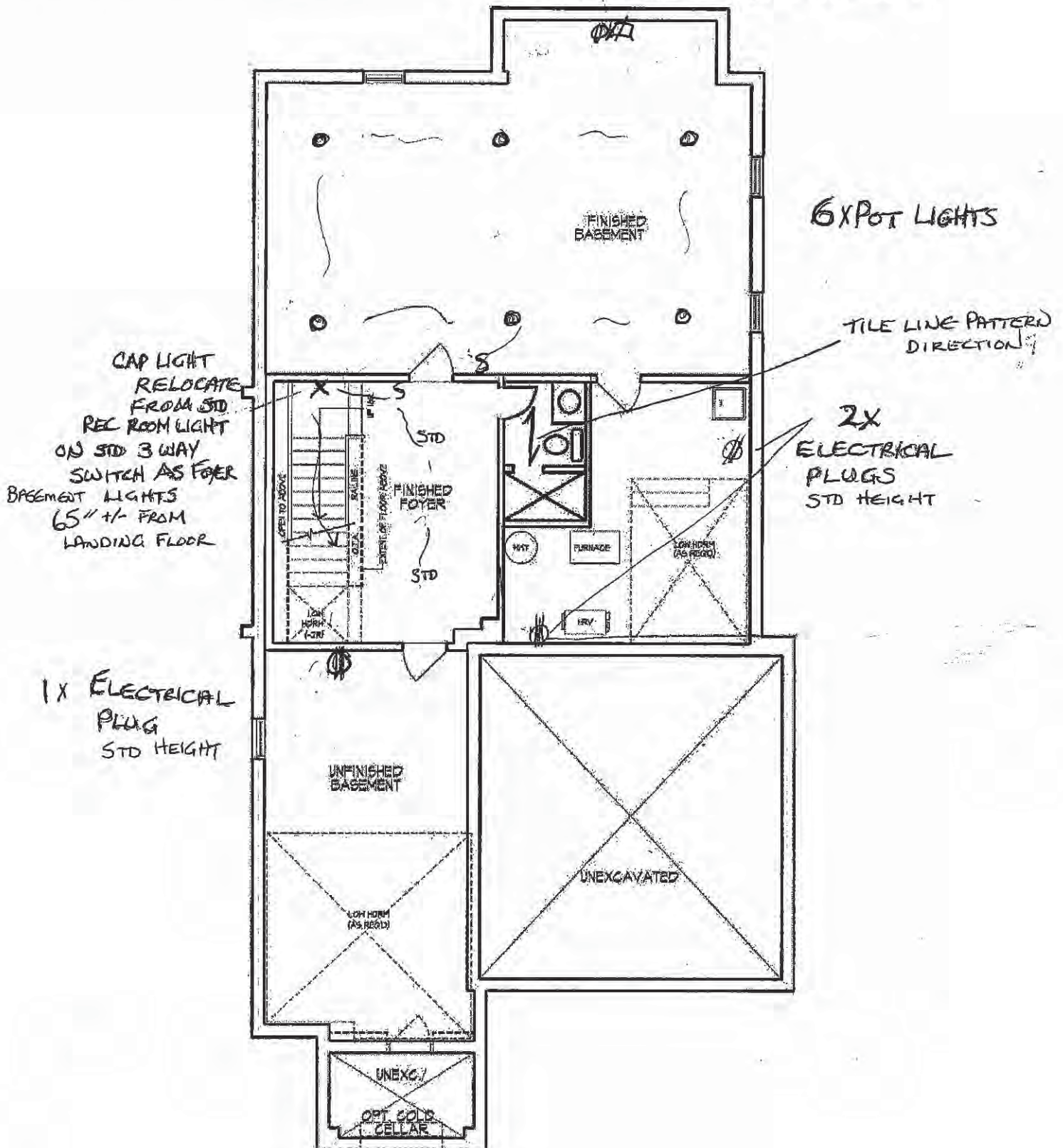
BASEMENT PLAN, ELEV. 'A' LOT (2)28
