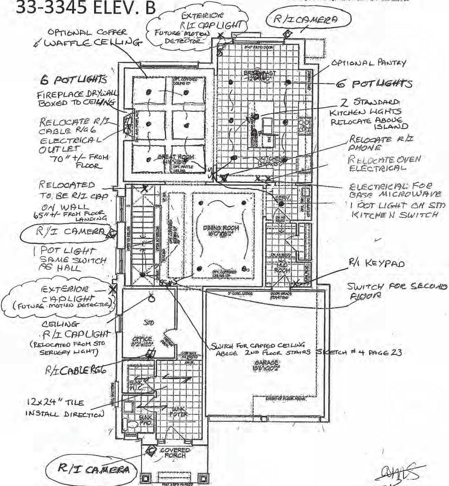
Ground Floor Plan – Elev. B Lot 228
