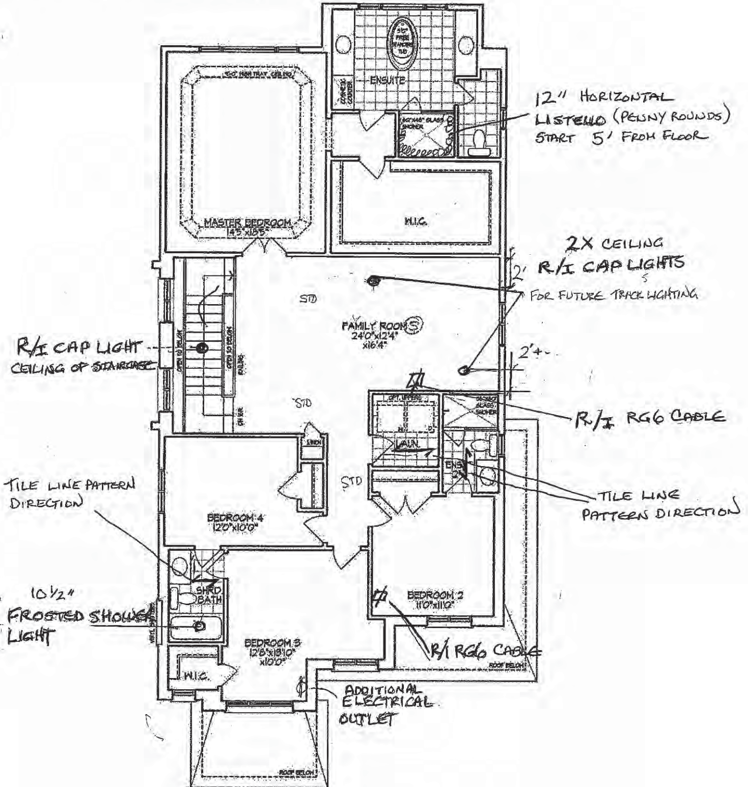
Second Floor Plan – Elev. B Lot 228
